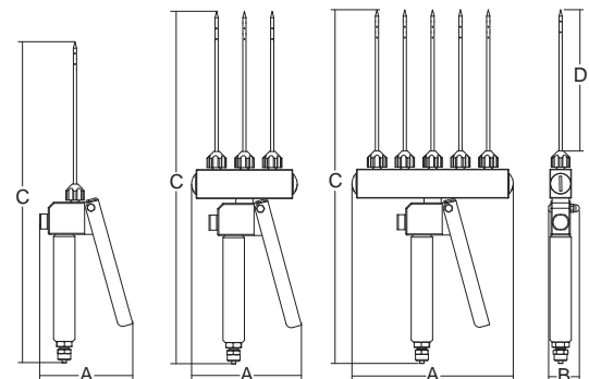
Dosatori da 1, 3 o 5 aghi Multiple needle heads with 1, 3 or 5 needles
